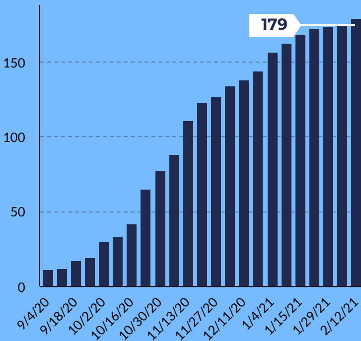
cumulative totals
