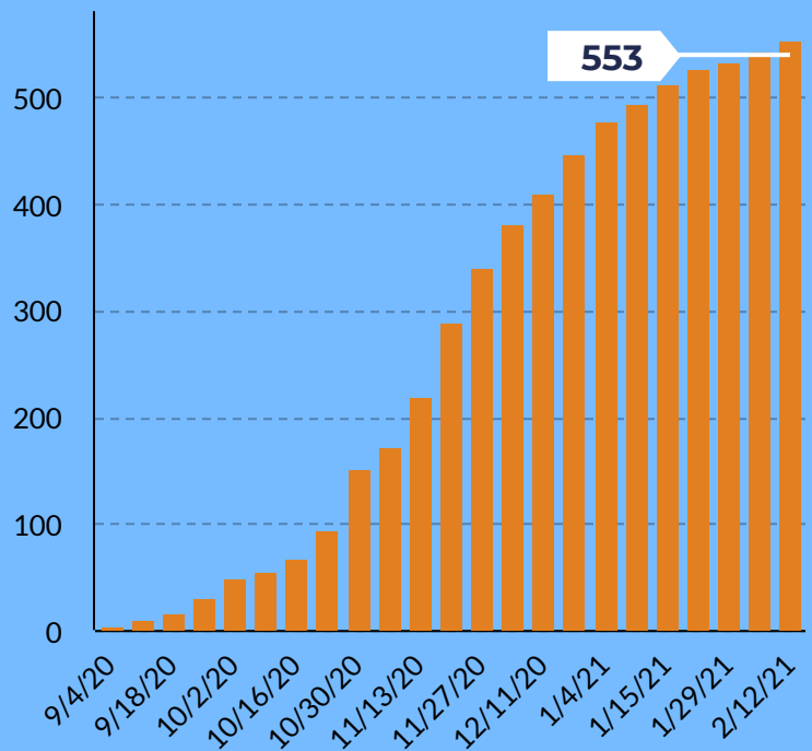
cumulative totals
